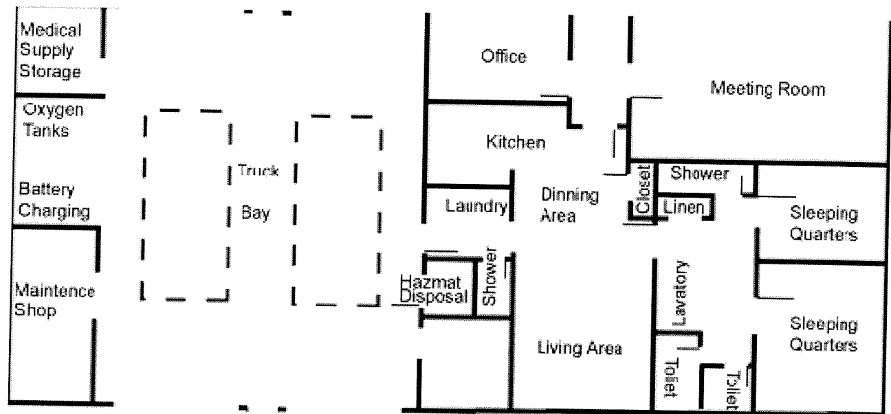
Figure 3. Example Floor Plan of a Two-Bay Building for an EMS System
