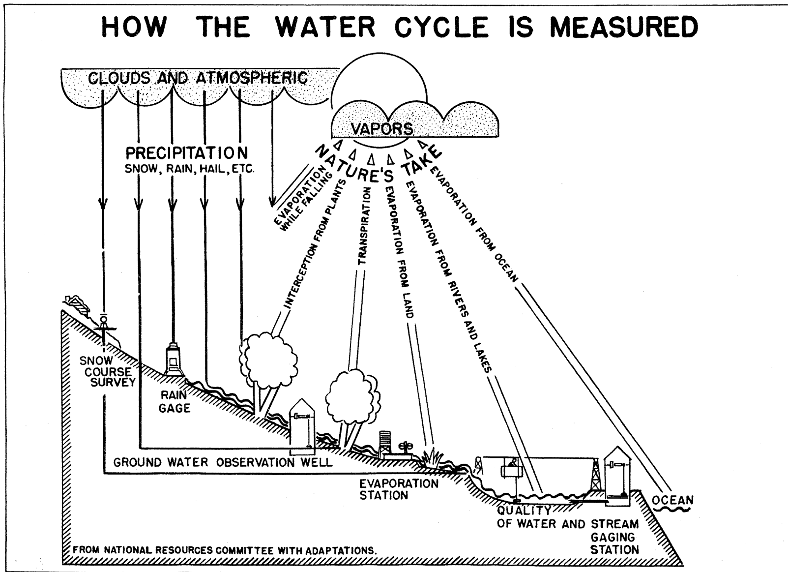
Figure 3.--Graphic representation of the hydrologic cycle
