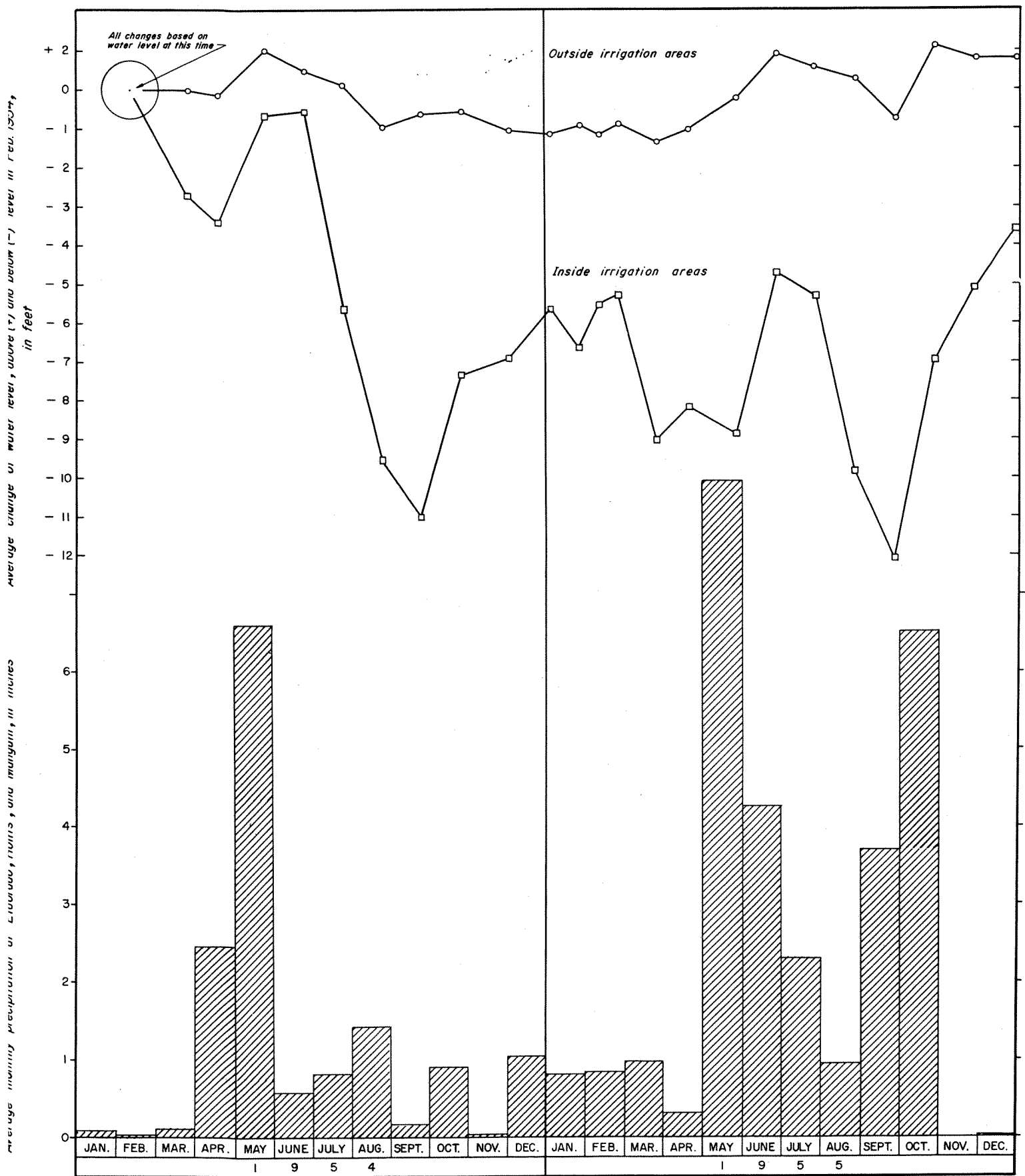
FIGURE 5-- Graphs showing average changes of water level in the Dog Creek Shale and Blaine Formation, Feb. 1954 to Dec. 1955, and average precipitation at Eldorado, Hollis, and Mangum.
