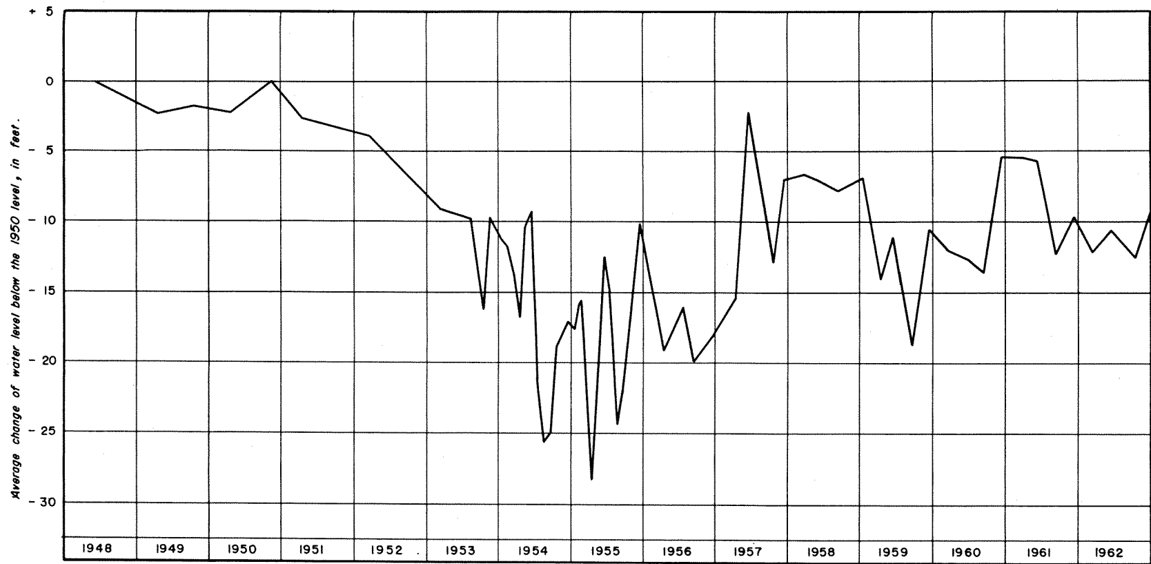
FIGURE 6-- Hydrograph showing average change of water level in eight observation wells based on the November 1950 level.
