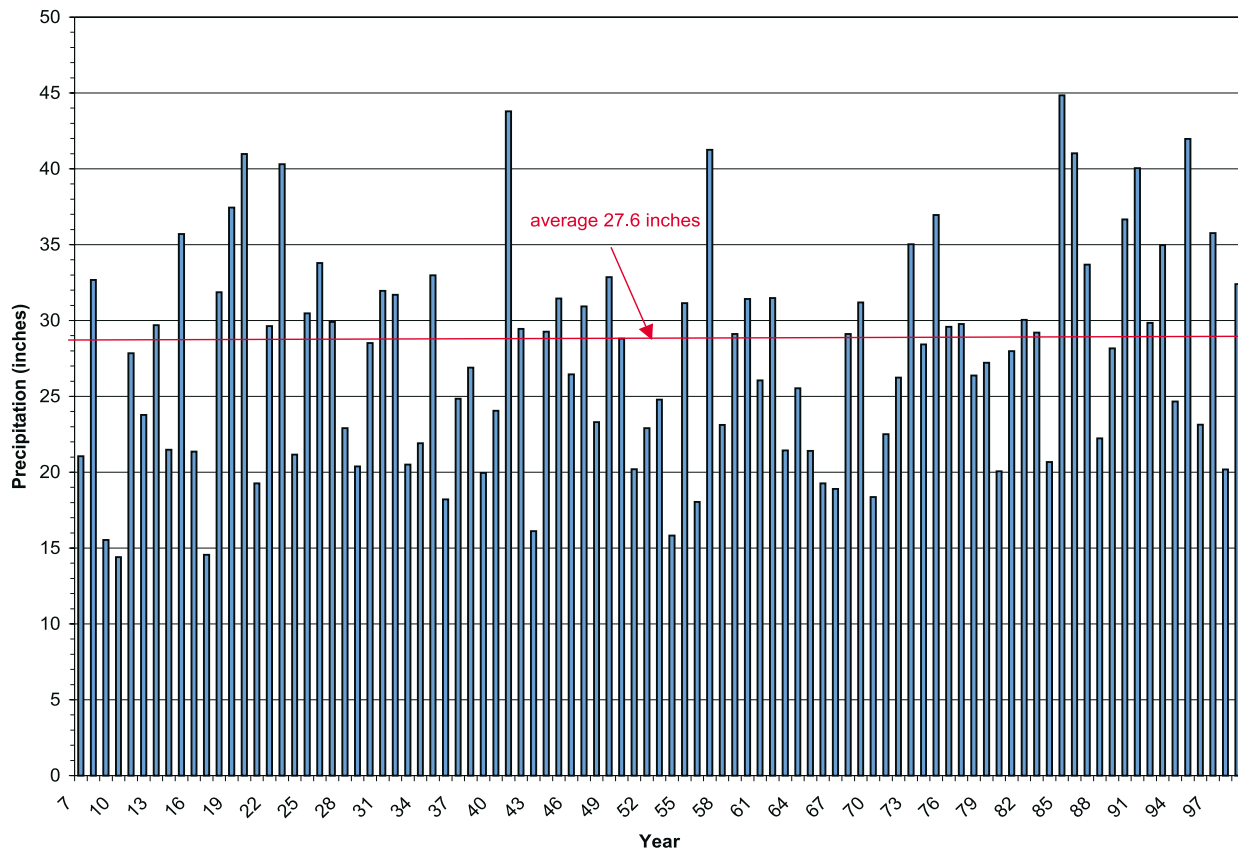
Figure 2. Annual precipitation measured at the Frederick gage from 1907 to 1999. Data from U.S. Department of Commerce, National Climatic Data Center and the Oklahoma Climatological Survey.
